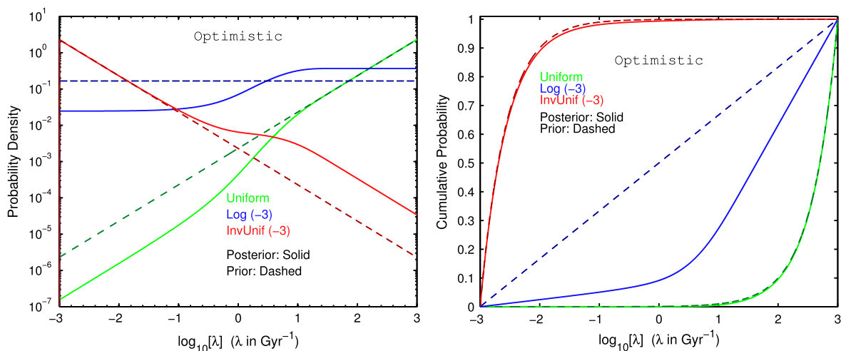
Fig. 1. PDF and CDF of \lambda for uniform, logarithmic, and inverse-uniform priors, for model optimistic, with \lambda_{\min} = 10^{-3} \text{ Gyr}^{-1} and \lambda_{\max} = 10^3 \text{ Gyr}^{-1} . ( Left ) The dashed and solid curves represent, respectively, the prior and posterior PDFs of \lambda under three different assumptions about the nature of the prior. The green curves are for a prior that is uniform on the range 0 \text{ Gyr}^{-1} \leq \lambda \leq \lambda_{\max} (uniform); the blue are for a prior that is uniform in the log of \lambda on the range -3 \leq \log \lambda \leq 3 [Log (-3)]; and the red are for a prior that is uniform in \lambda^{-1} on the interval 10^{-3} \text{ Gyr} \leq \lambda^{-1} \leq 10^3 \text{ Gyr} [InvUnif (-3)]. ( Right ) The curves represent the CDFs of \lambda . The ordinate on each curve represents the integrated probability from 0 to the abscissa (color and line-style schemes are the same as in Left ). For a uniform prior, the posterior CDF traces the prior almost exactly. In this case, the posterior judgment that \lambda is probably large simply reflects the prior judgment of the distribution of \lambda . For the prior that is uniform in \lambda^{-1} (InvUnif), the posterior judgment is quite opposite—namely, that \lambda is probably quite small—but this judgment is also foretold by the prior, which is traced nearly exactly by the posterior. For the logarithmic prior, the datum (that life on Earth arose within a certain time window) does influence the posterior assessment of \lambda , shifting it in the direction of making greater values of \lambda more probable. Nevertheless, the posterior probability is approximately 12% that \lambda < 1 \text{ Gyr}^{-1} . Lower \lambda_{\min} and/or lower \lambda_{\max} would further increase the posterior probability of very low \lambda , for any of the priors.
