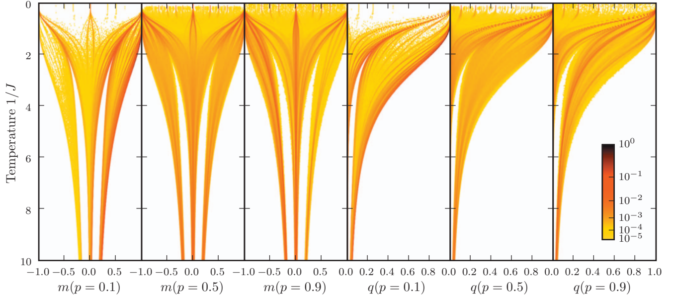
FIG. 1. (Color) Local-order-parameter tulips: probability distributions of local magnetization (left panels) and spin-glass order parameters of the interior sites on an Apollonian network with Ising spin-glass interactions, as a function of temperature, for three different antiferromagnetic bond concentrations p .
